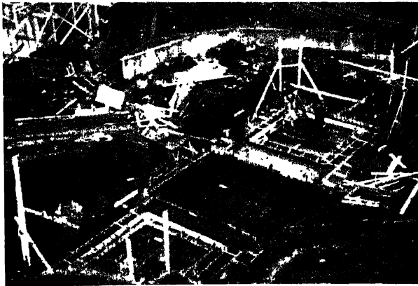
Fig. 175. —Construction of Base of Pier, Inverbervie Bridge.
